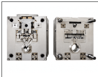
Pressure Die Casting Dies
